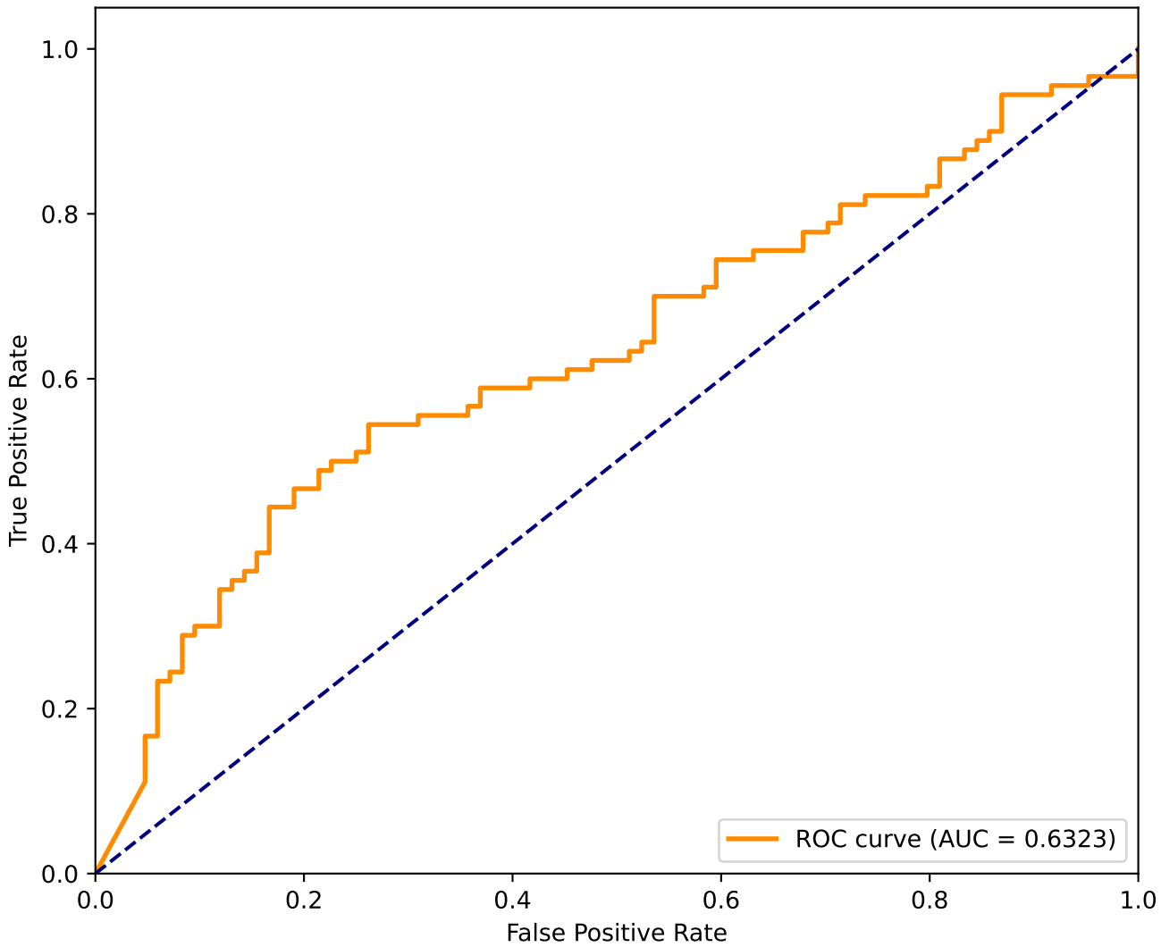
ROC Curve - KNN
